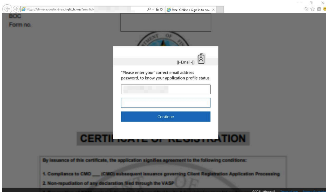
Figure 5: Credential capture landing page.
