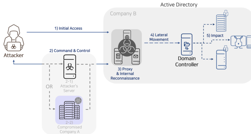
Figure 2. Summary diagram of Dalbit group's infiltration process
