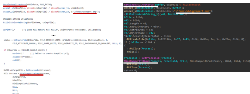
Figure 7. Left (open-source Dumpert) vs. right (Dumper used by the Dalbit group)
