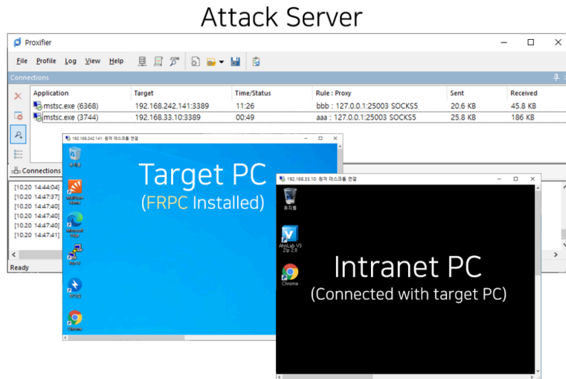
Figure 4. Example of Socks5 usage
