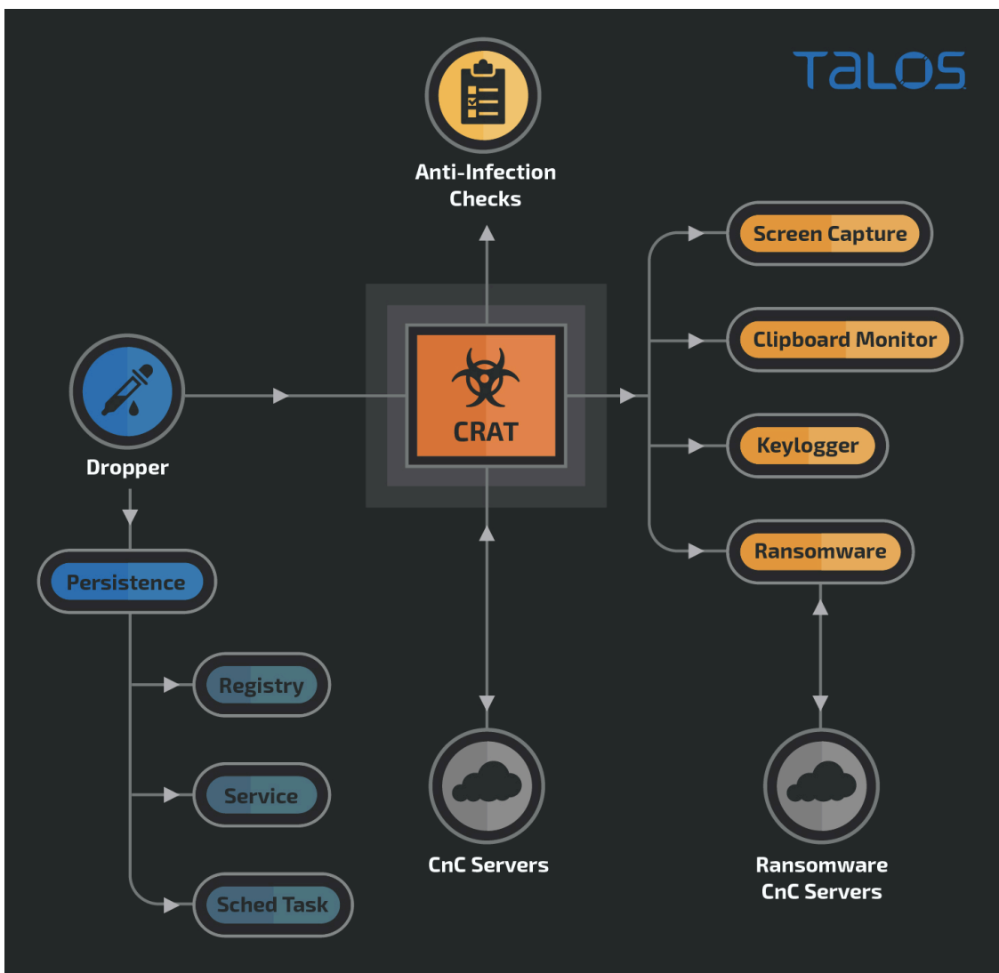
Infection chain of CRATv2
