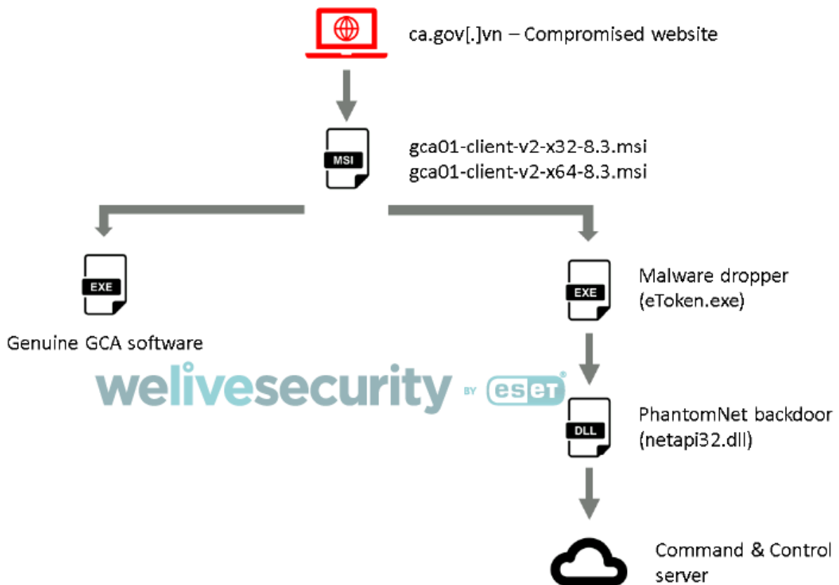
Figure 3. Simplified scheme of the supply-chain attack.
