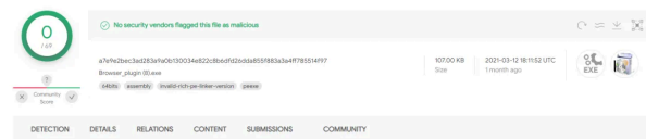
Figure 8: VT hit
