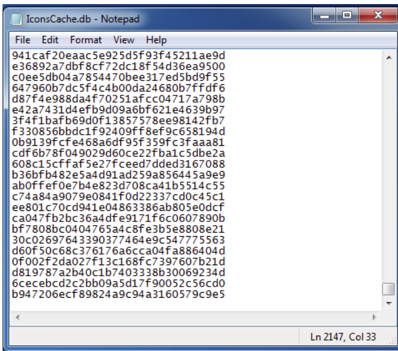
Figure 9. IconsCache.db contents.
