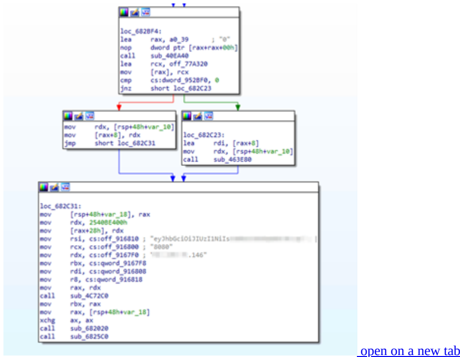
Figure 8. The address and access token being passed as compilation flags and hardcoded inside the RAT client
