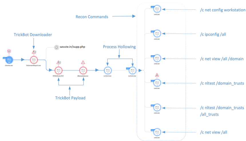
Figure 6. Cortex XDR causality chain
