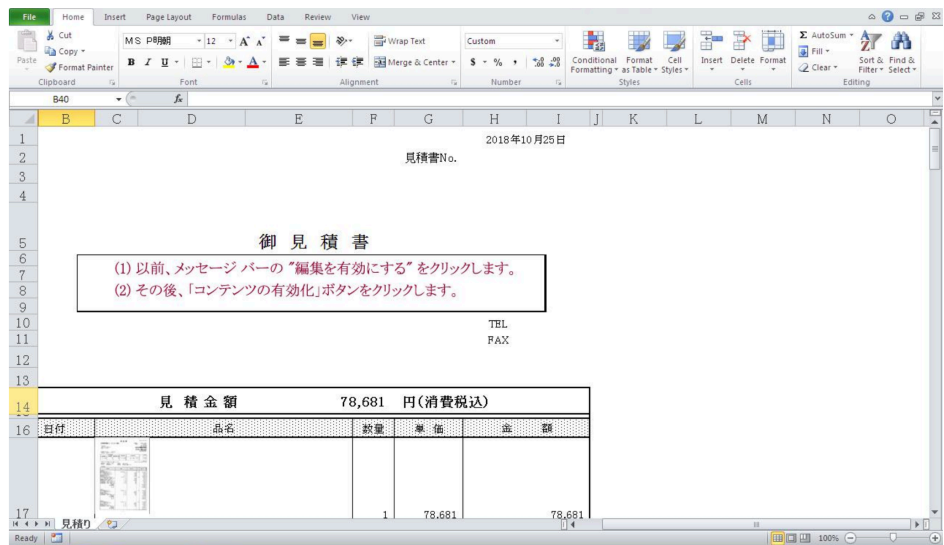
Figure 1. Screenshot of Malicious, Macro-enabled Microsoft Excel Document Upon opening the Excel document and enabling macros, the victim machine begins to run through the series of events detailed below.
