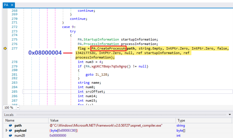
Figure 4.2 – Creating a suspended process
