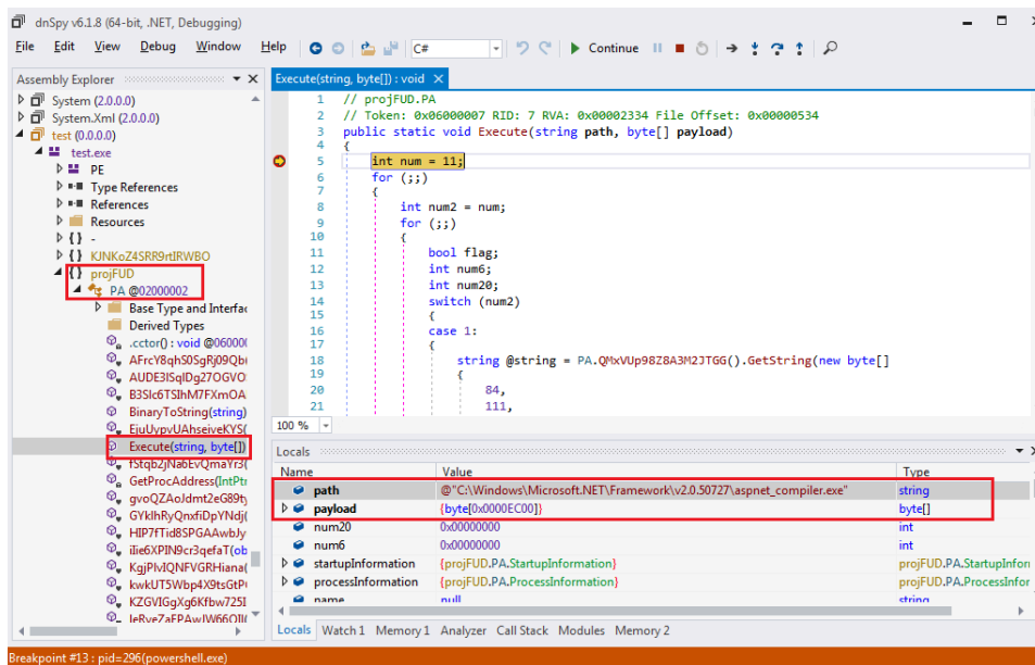
Figure 4.1 – Break at the entry of function “projFUD.PA.Execute()”
