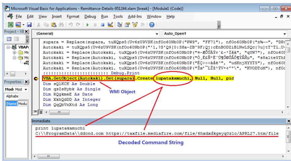
Figure 2.2 – The WMI object used to execute a decoded command
