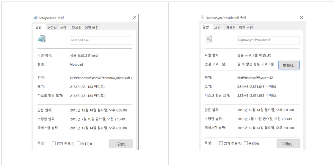
Figure. Timestamp comparison of a default system file (notepad.exe) and malware (DapowSyncProvider.dll)
