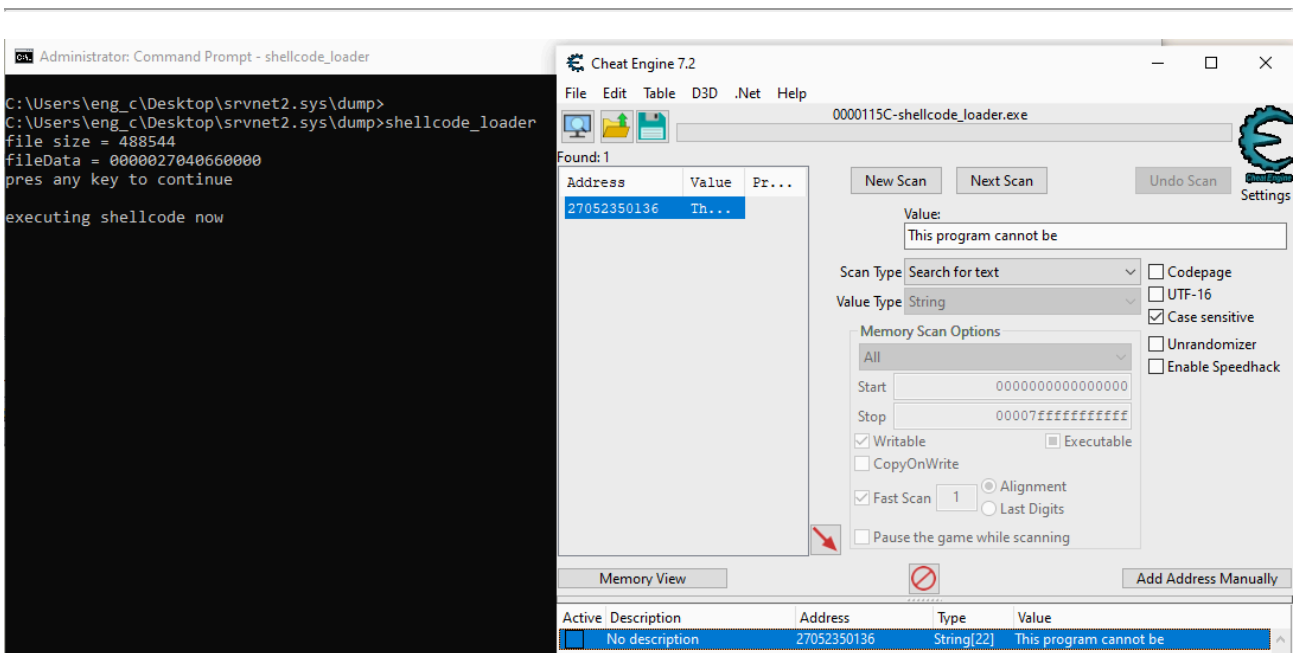
Figure 23: Running the shellcode using the C program and finding the unpacked .NET PE
