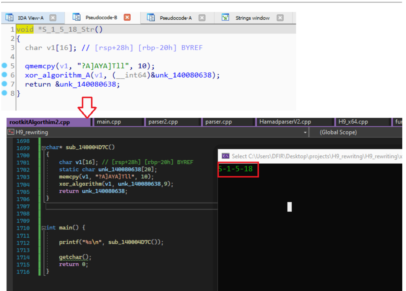
Figure 17: Get token SID and compare it with string “S-1-5-18”
