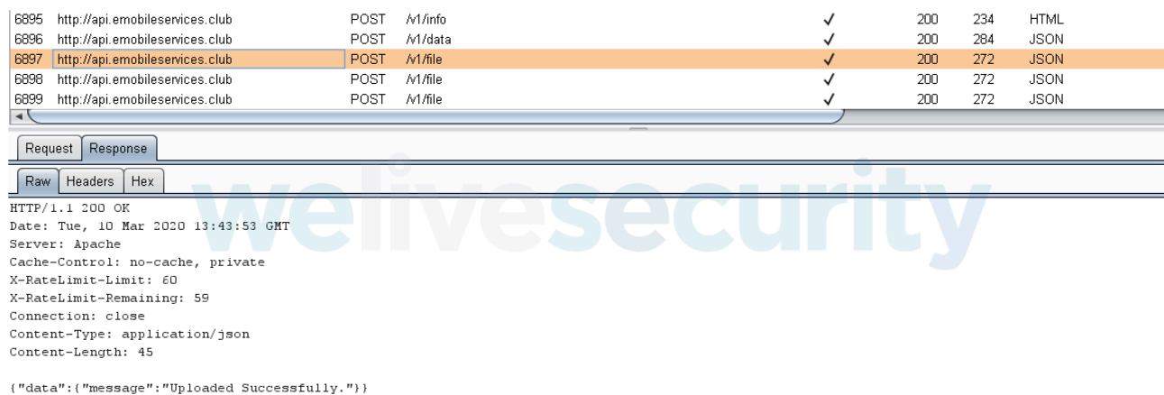
Figure 6. The victim’s device uploads the user data to the app’s server
