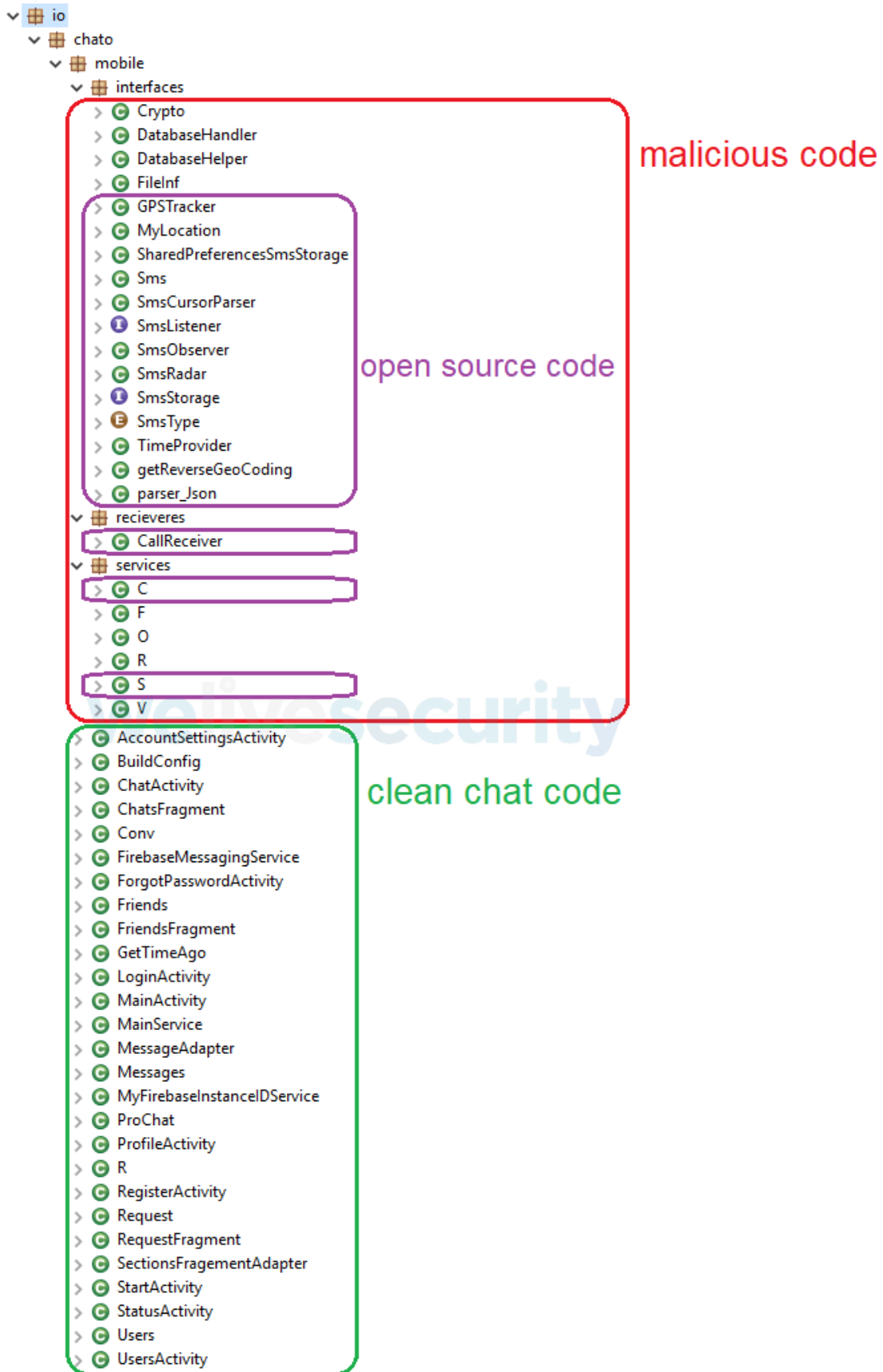
Figure 5. The developer used different pieces of open source code to create the malicious app
