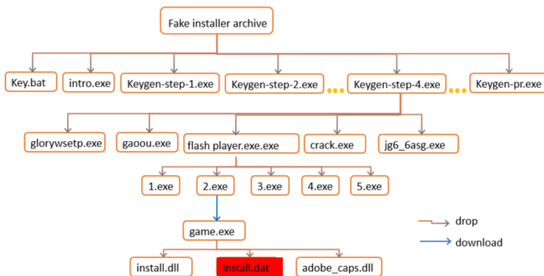
Execution flow, variant 1
