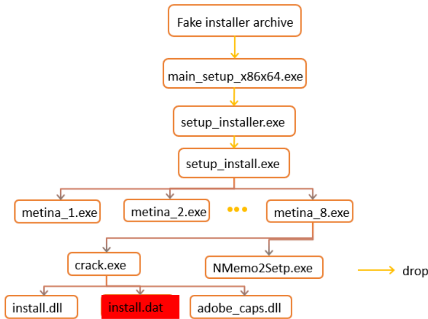
Execution flow, variant 2
