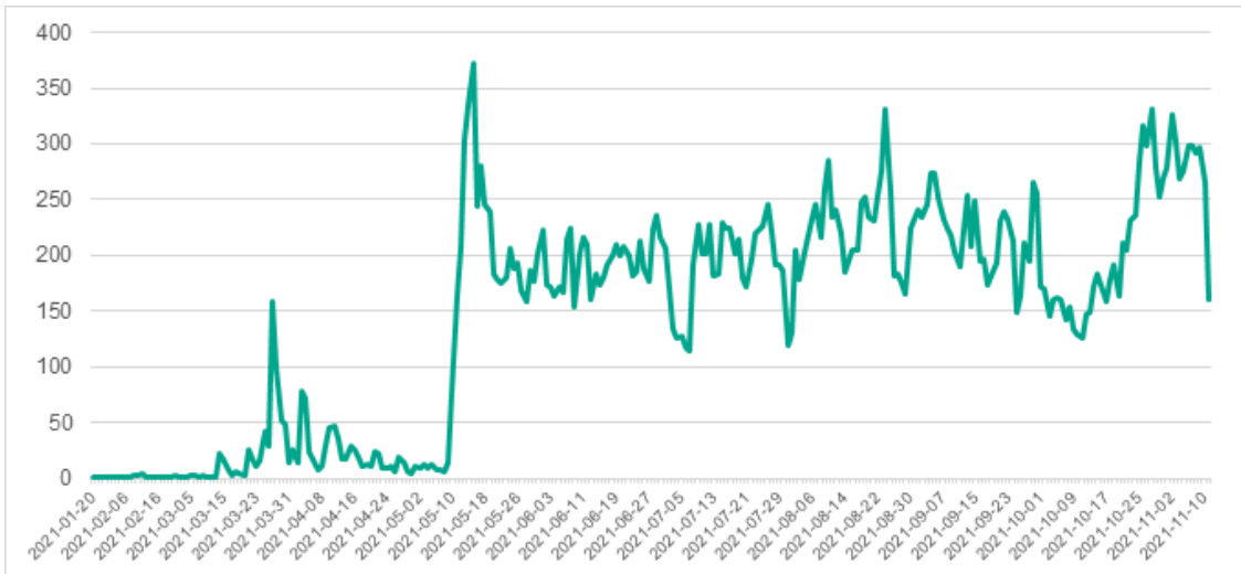
Number of systems on which PseudoManuscript was detected, by day
