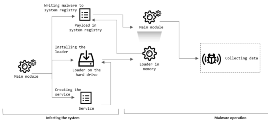
Malware installation and execution
