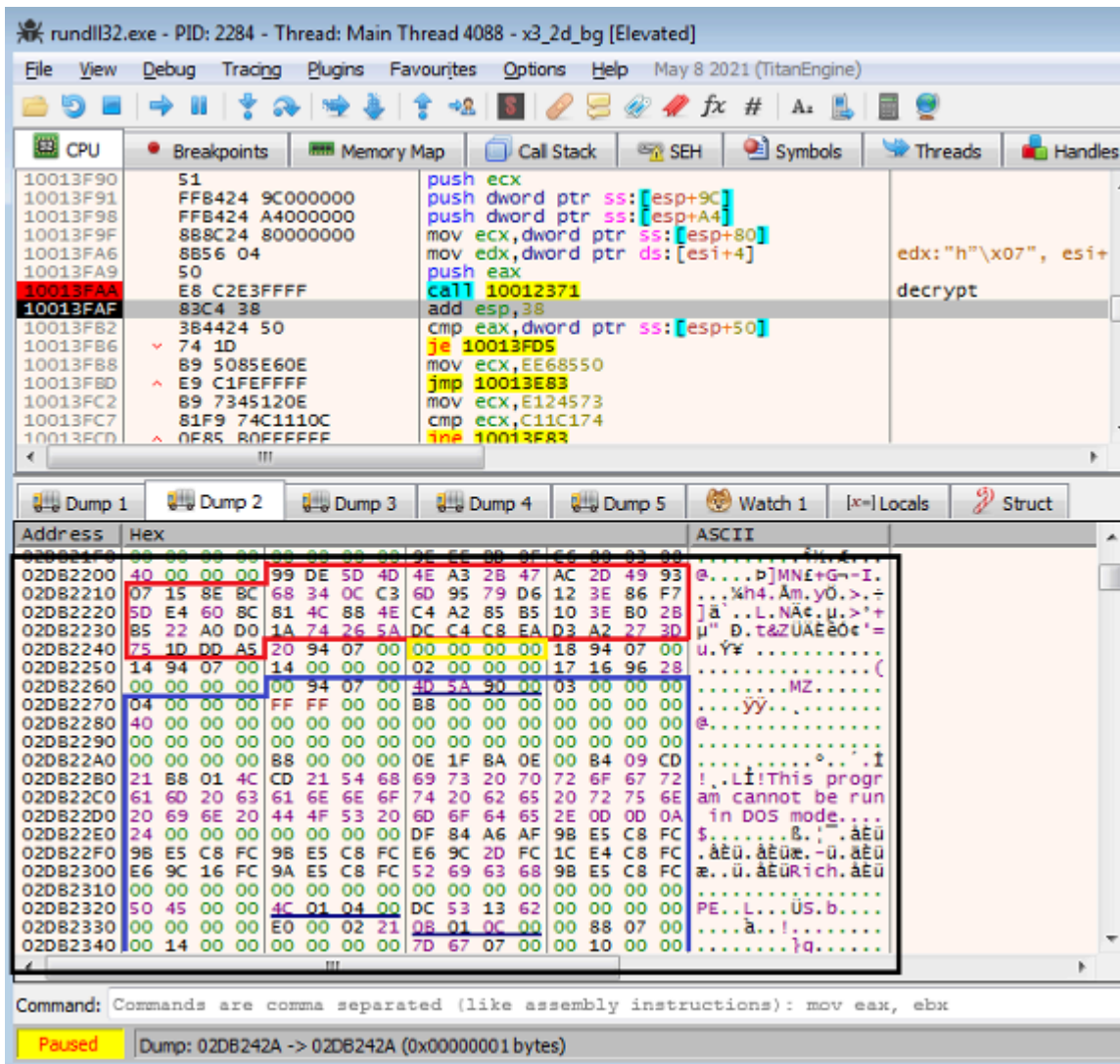
Figure 1.1 – A decrypted module in the packet
