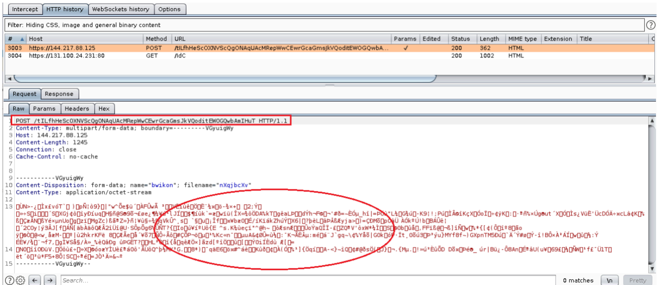
Figure 6.2 – Display of a captured packet to C2 server with encrypted data
