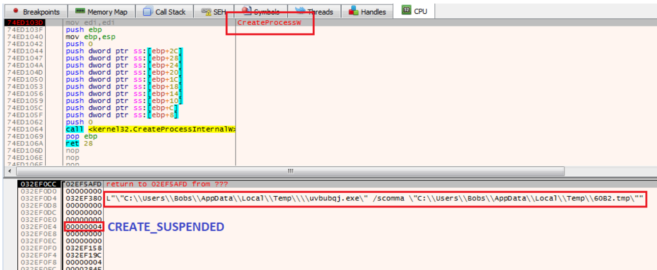
Figure 2.1 – Call API CreateProcessW() to create a suspended process
