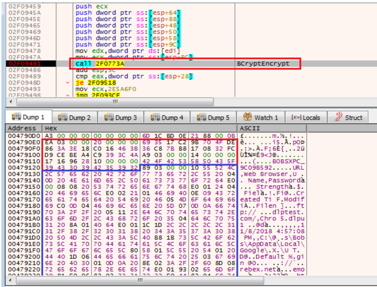
Figure 6.1 – Call BCryptEncrypt() to encrypt the stolen data
