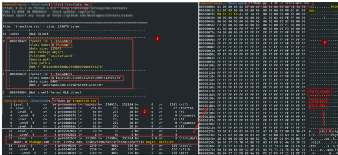
Figure 5 – Embedded payload in RTF file
