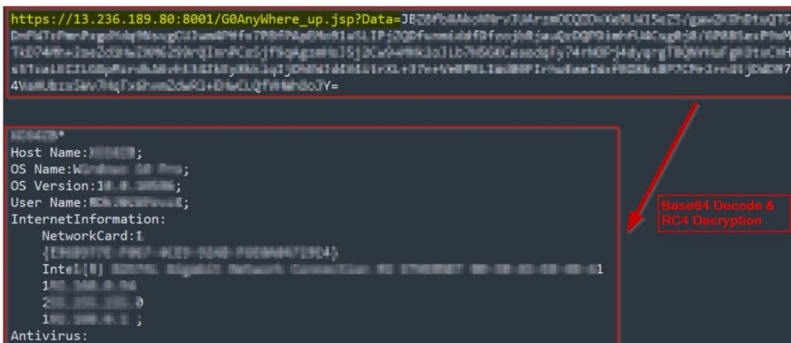
Figure 7 – Exfiltrated data to C&C server
