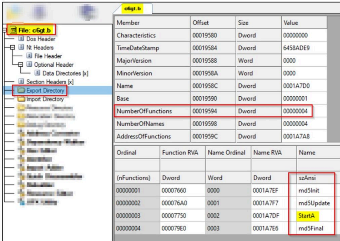
Figure 6 – Export functions of the DLL loader
