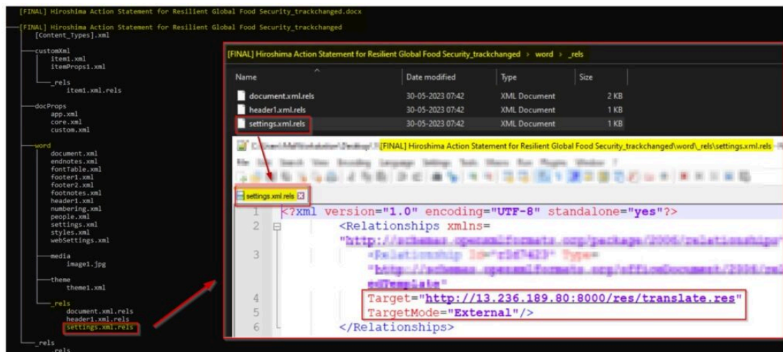
Figure 4 – Payload URL present inside the XML file of the malicious document
