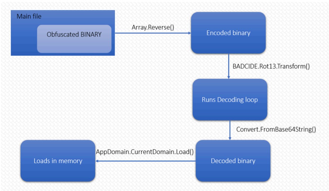
Figure 5: Binary decoding process
