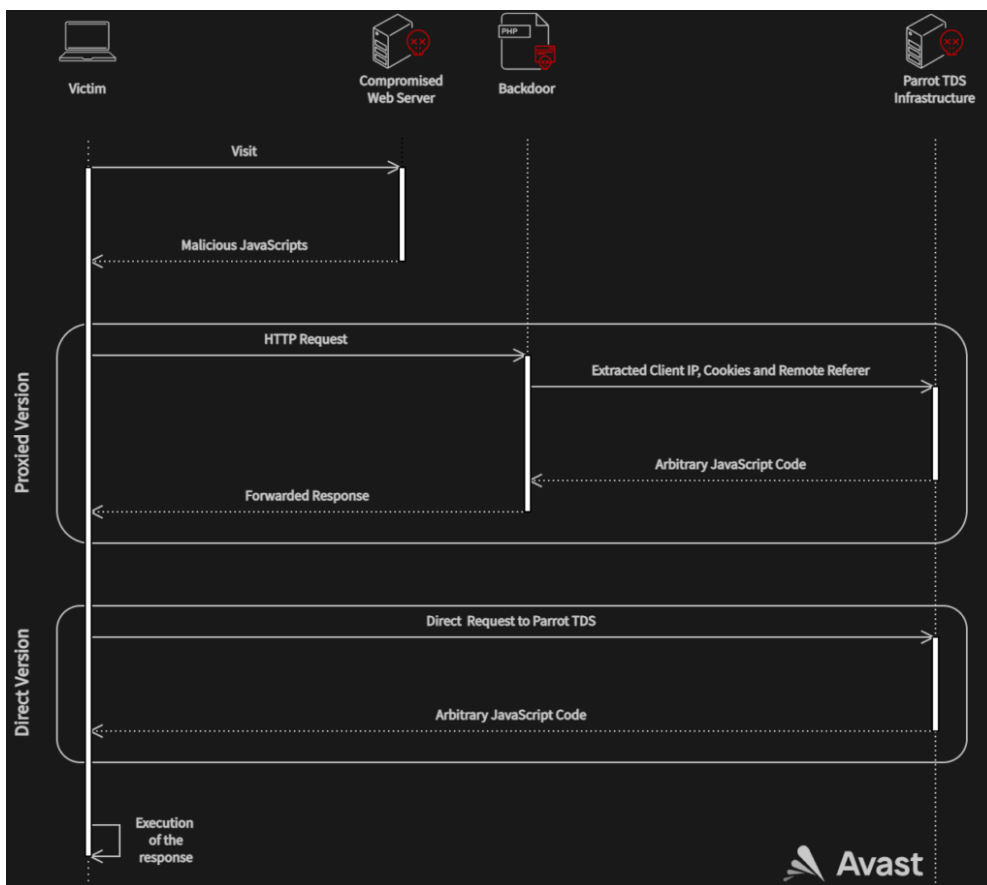
Parrot's direct and proxied forwarding (Avast)
