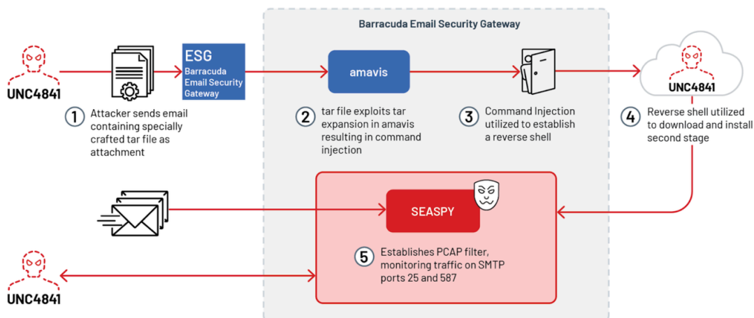
Figure 3: SEASPY attack path
