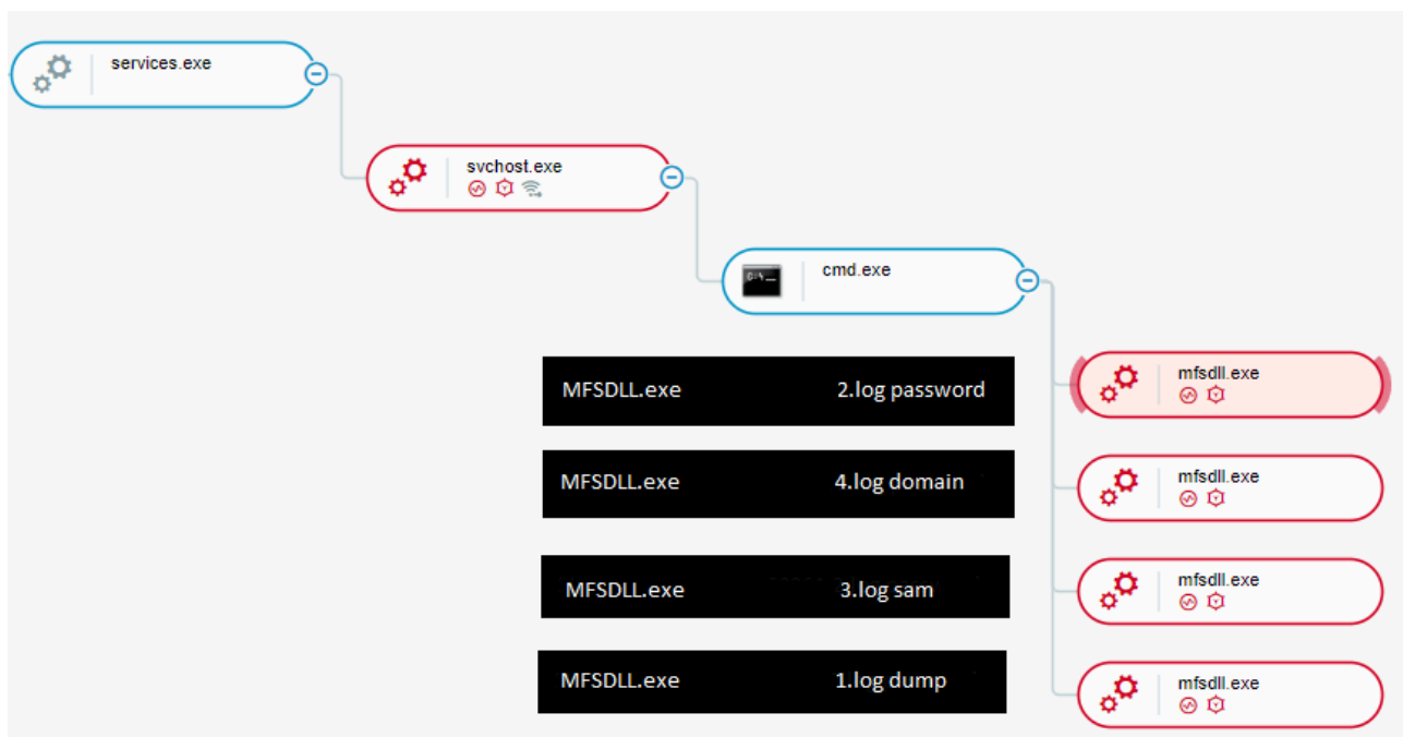
MFSDLL.exe executions as seen in the Cybereason XDR Platform
