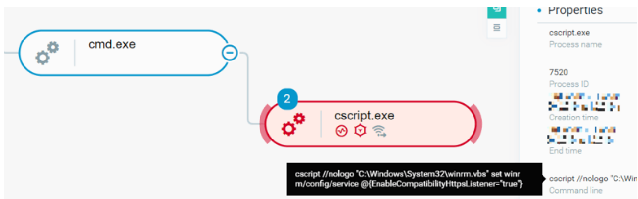
Modifying system WinRM configuration using cscript.exe as seen in the Cybereason XDR Platform
