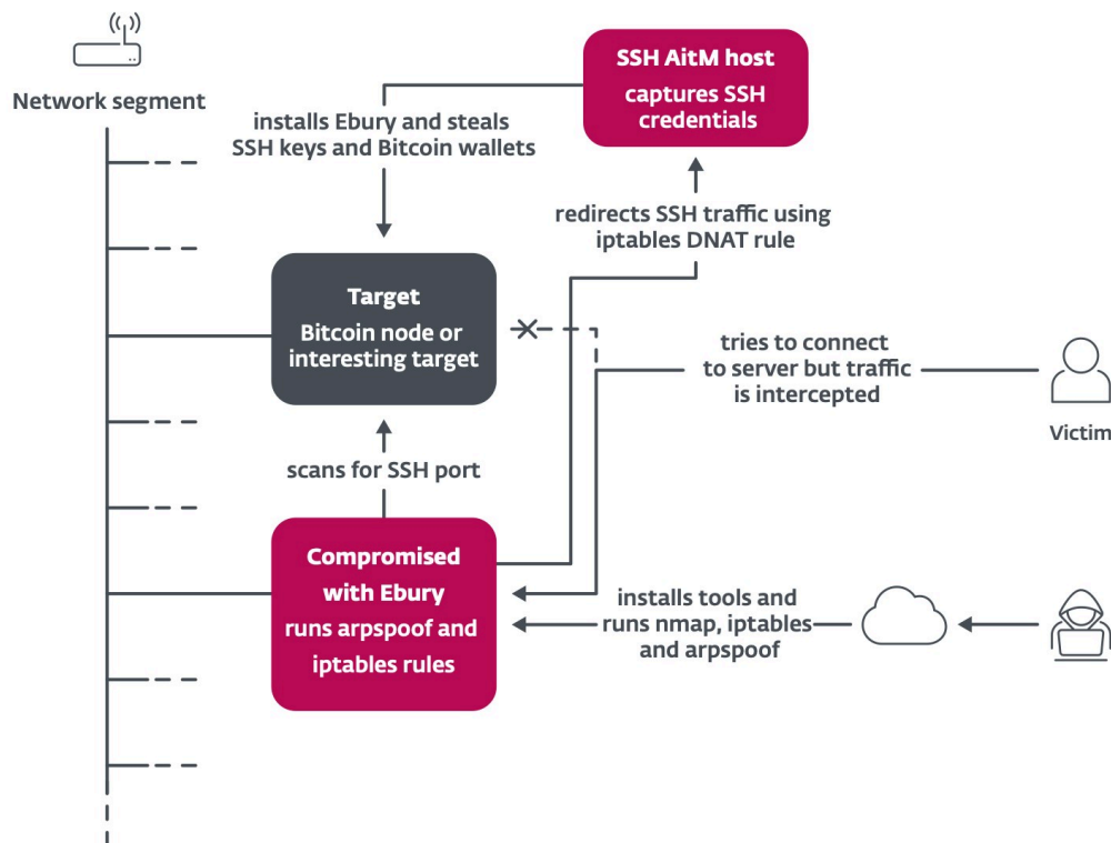
Figure 3. Overview of AitM attacks perpetrated by the Ebury gang
