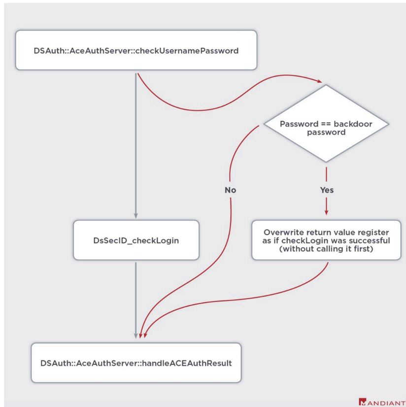
Figure 4: ACE Auth Bypass Variant
