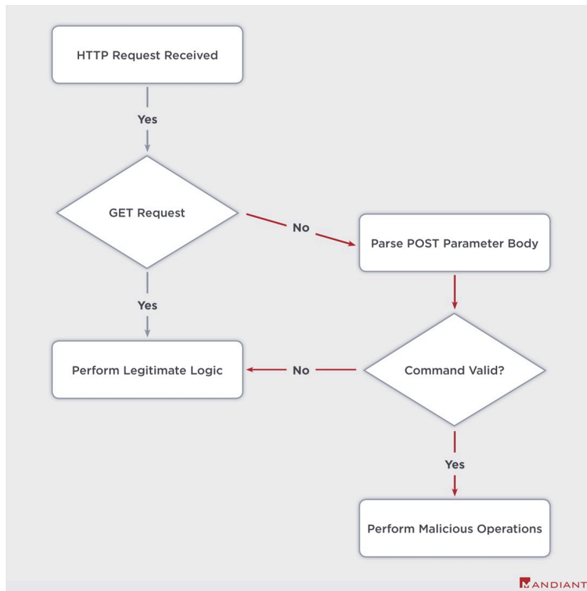
Figure 7: Webshells respond to POSTs
