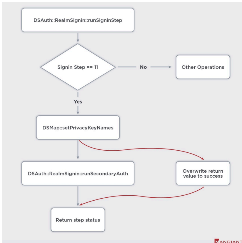
Figure 5: RealmSignIn 2FA Auth Bypass
