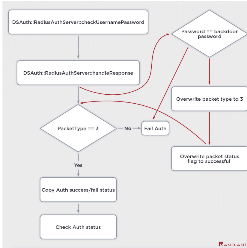
Figure 2: Radius-2FA Bypass
