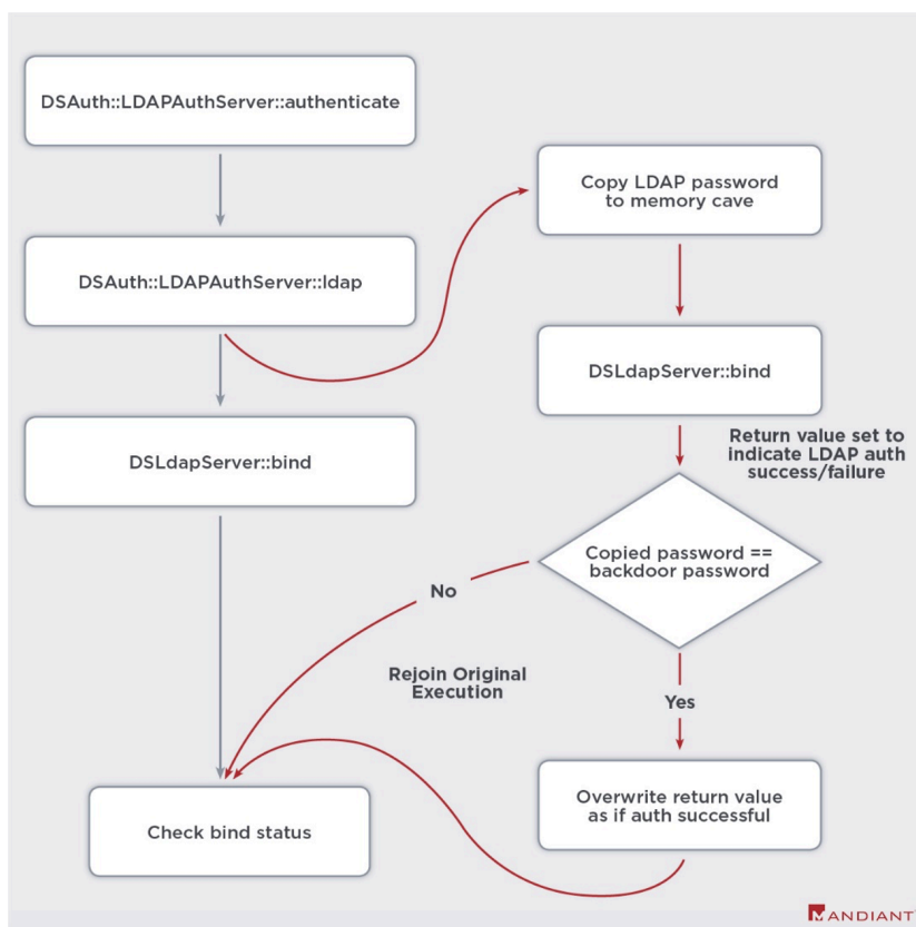
Figure 1: LDAP Auth Bypass
