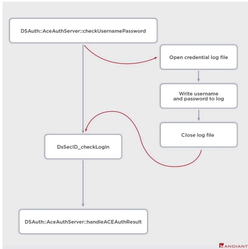
Figure 3: ACE Auth Credential Log
