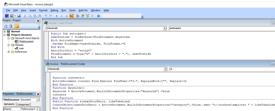
Figure 9: Macro code to deobfuscate HTML code
