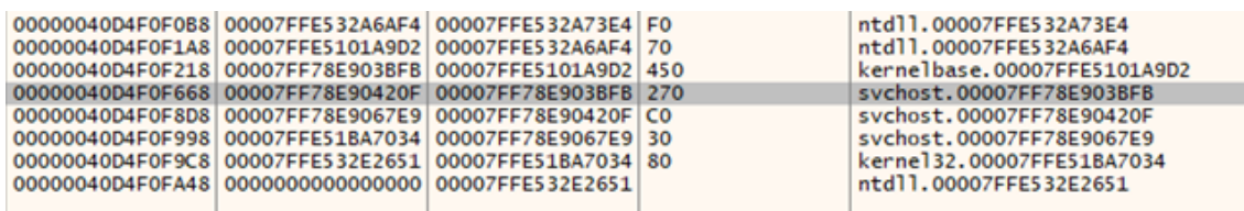
Figure 2. Call stack before stack swap, LoadLibraryExW in kernelbase returning to svchost.exe ( 0x7FF78E903BFB )
