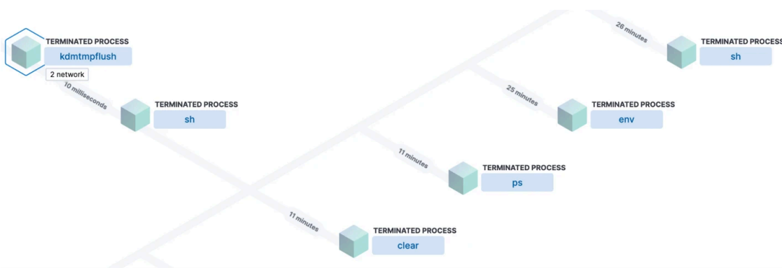
Elastic Analyzer View of BPFDoor following a reverse shell connection and post exploitation actions
