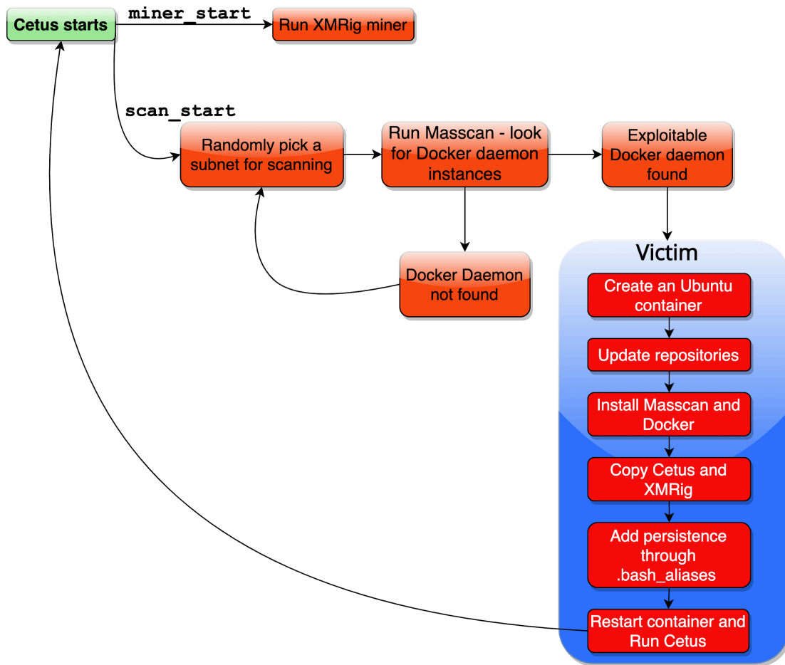
Figure 1. Cetus life cycle.
