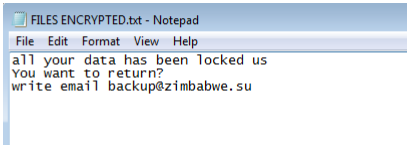
Figure 5: FILES ENCRYPTED.txt
