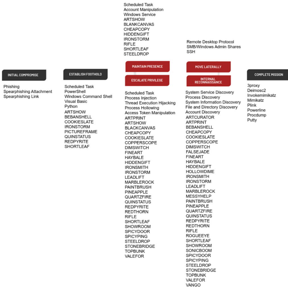
Figure 5: Attack Lifecycle
