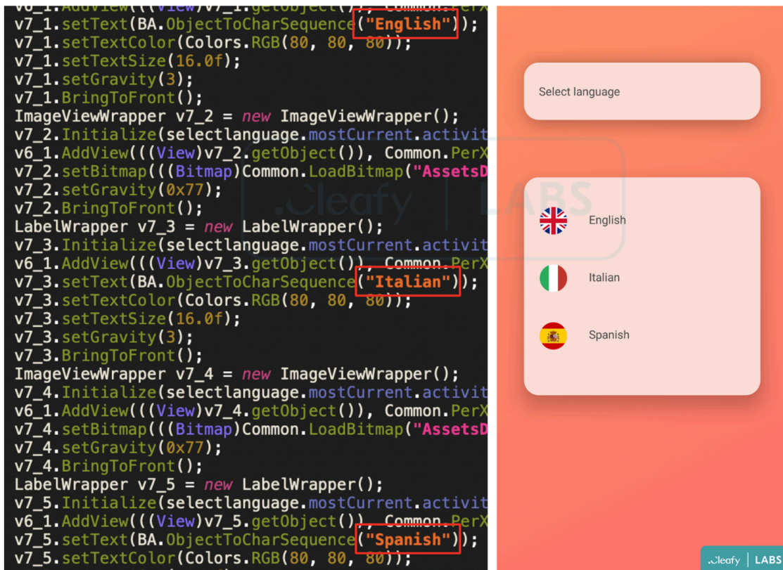
Figure 11 – SMS stealer targeted countries
