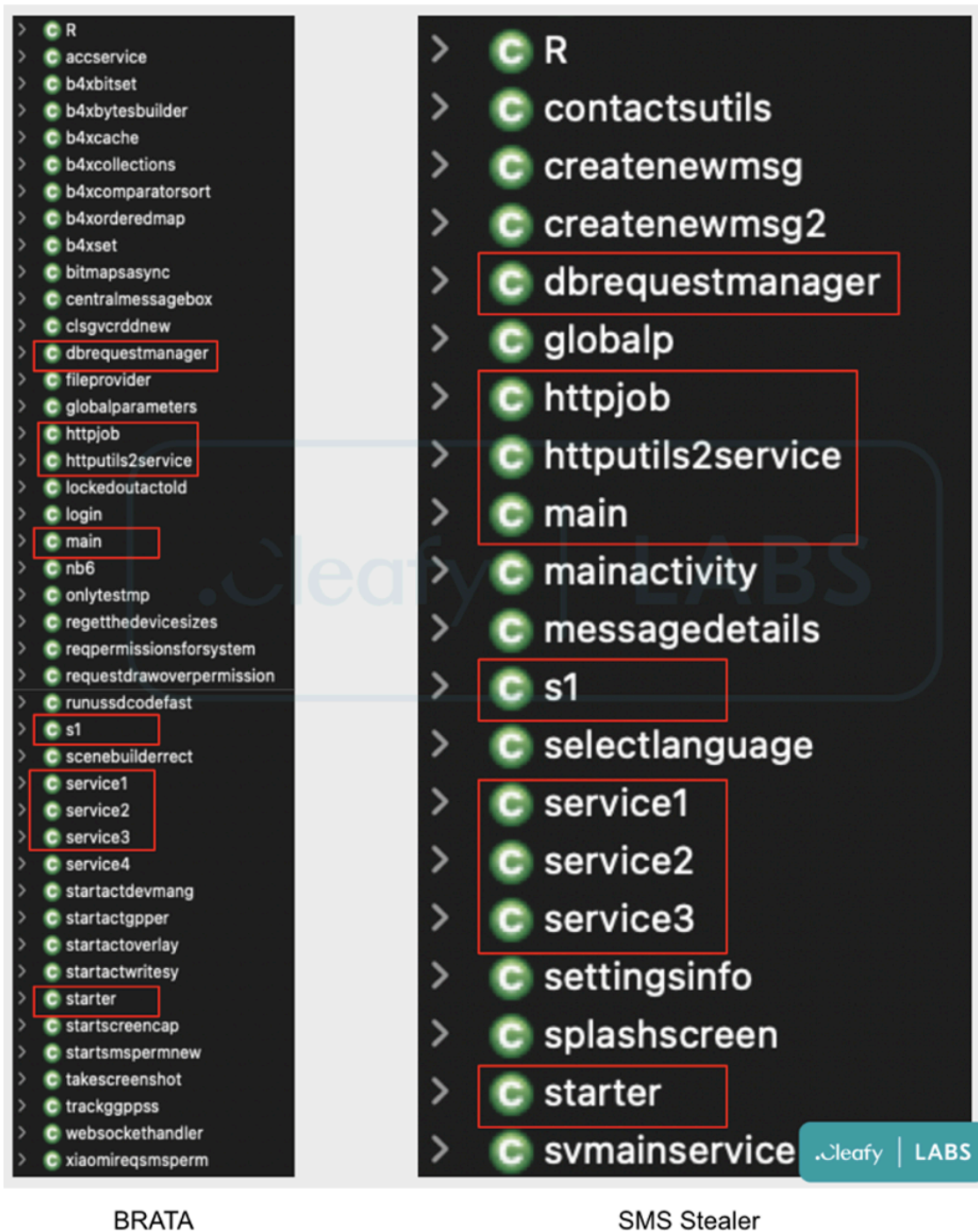
Figure 9 – Names similarities between BRATA and the SMS stealer
