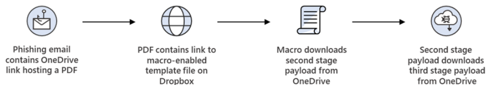
Figure 2. Template injection technique
