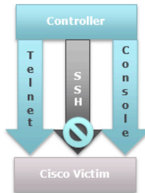
Figure 2: Backdoor Access
