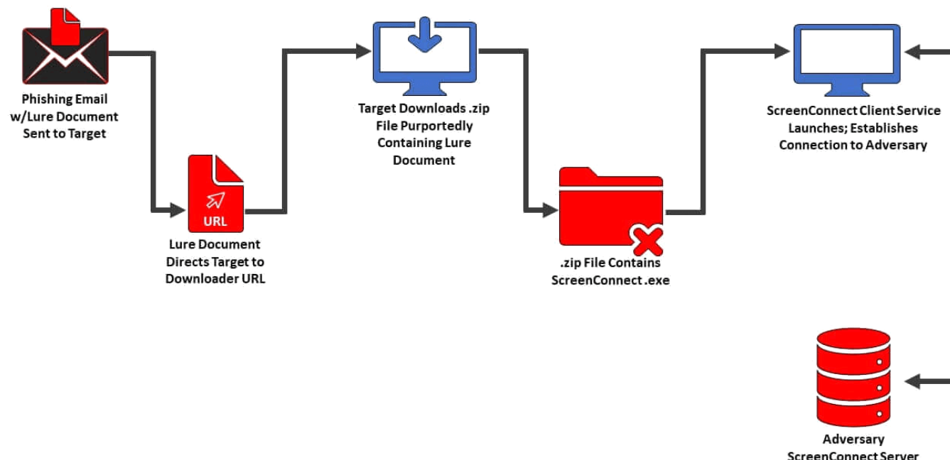
Figure 1 - Static Kitten Campaign Infection Chain
