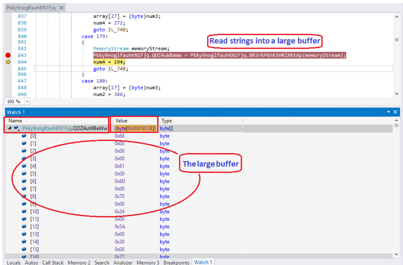
Figure 10. Reading strings in the large buffer
