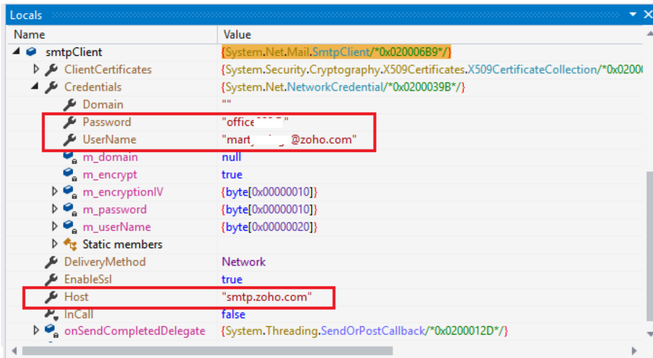
Figure 12. Attacker’s SMTP credential
