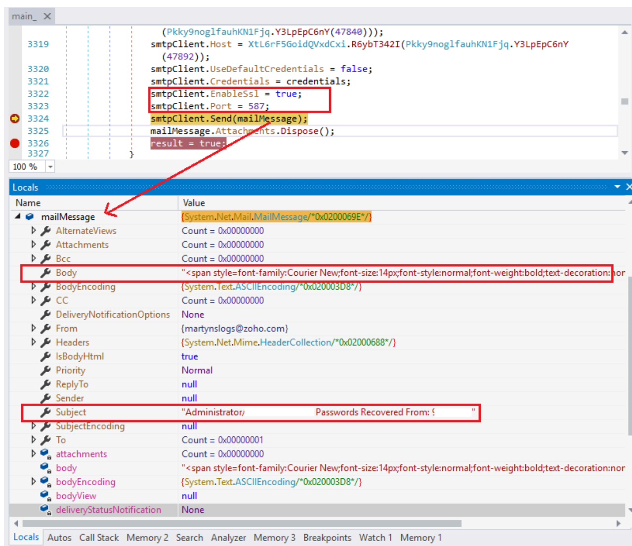
Figure 11. Email content with collected data
