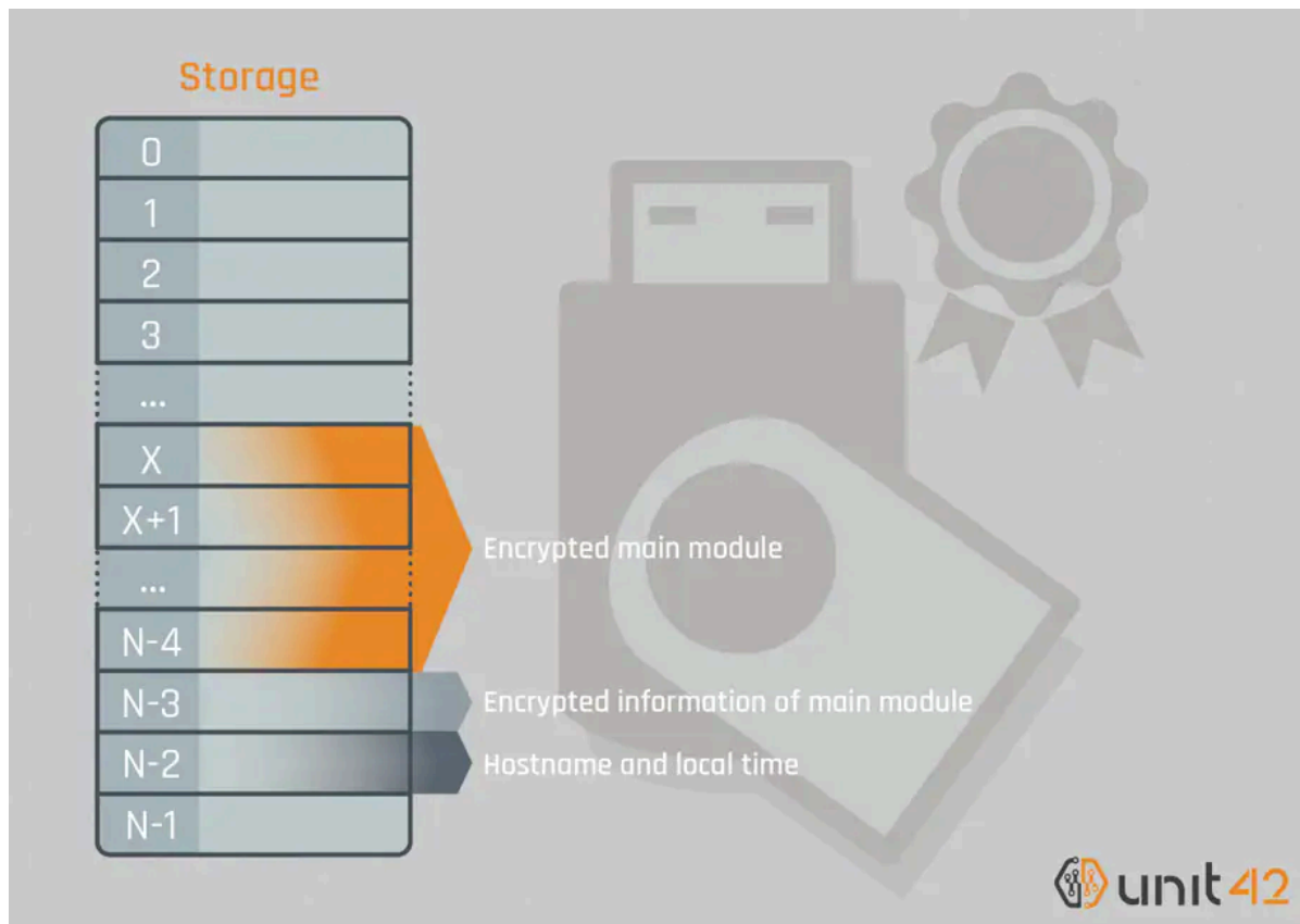
Figure 5 Data layout on the malicious storage
