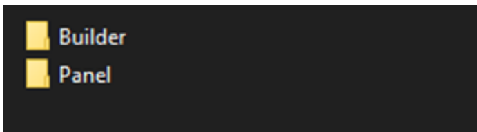
Figure 4 – Leaked Files
