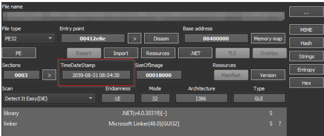
Figure 7 – File Details
