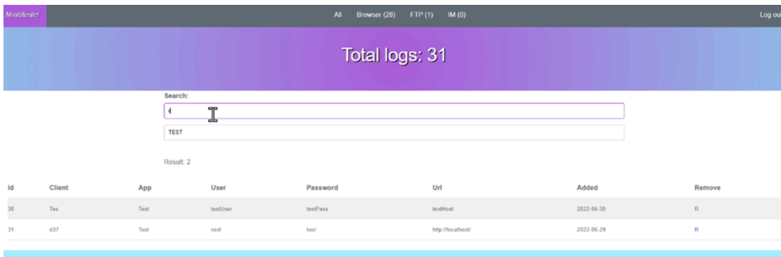
Figure 6 – MiniStealer panel
