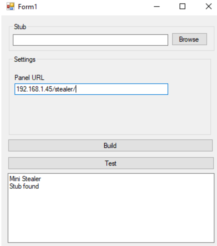
Figure 5 – MiniStealer Builder
