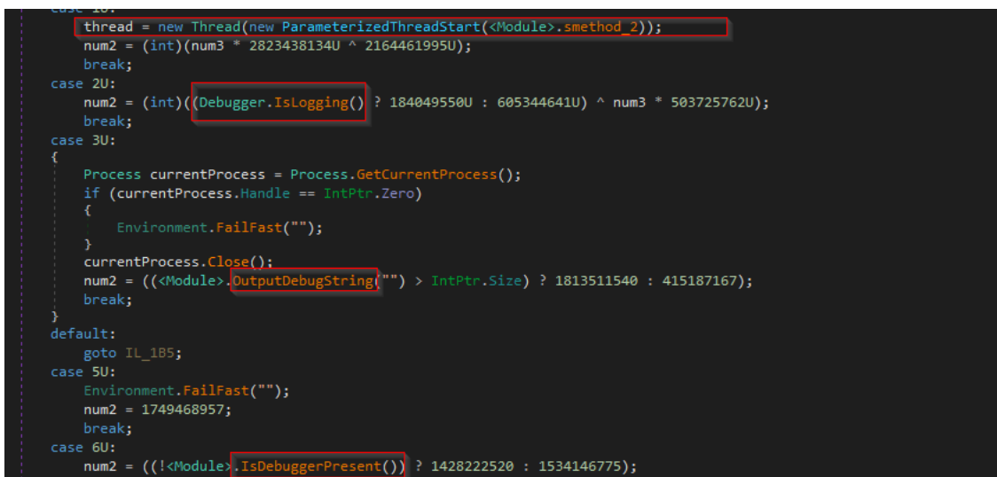
Figure 9 – Anti-Analysis
