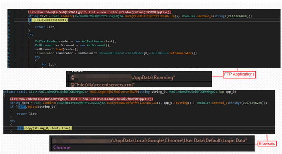
Figure 10 – Stealing Data
