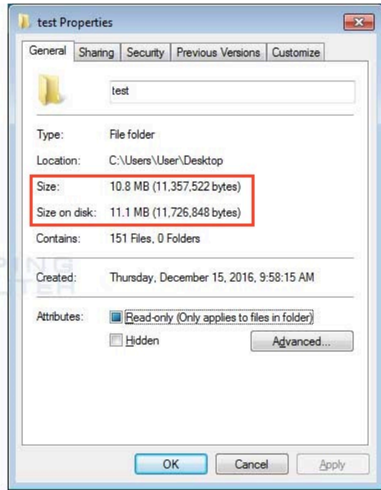
After Encryption
