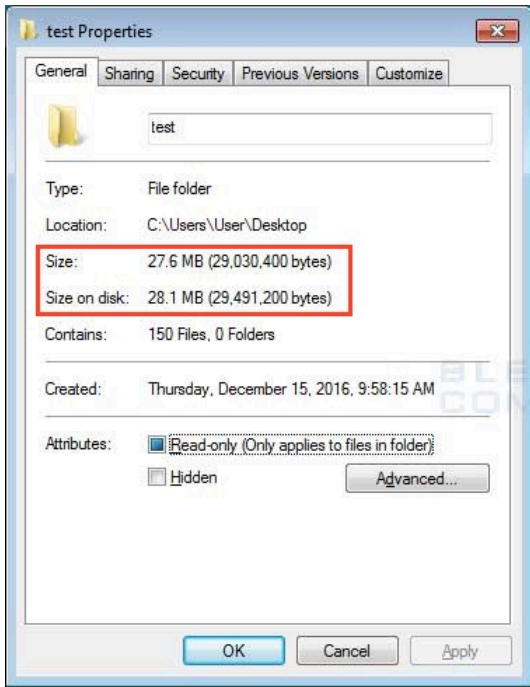
Before Encryption
