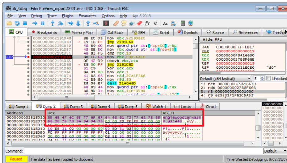
Figure 3.1. A display of the decrypted host string of the C2 server
