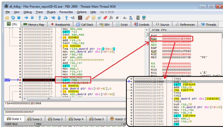
Figure 2.3. Calling the OEP of the deployed PE file
