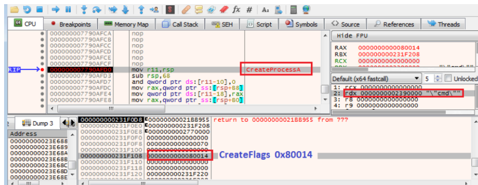
Figure 3.4. Creating the “cmd.exe” process by calling the API CreateProcessA()
