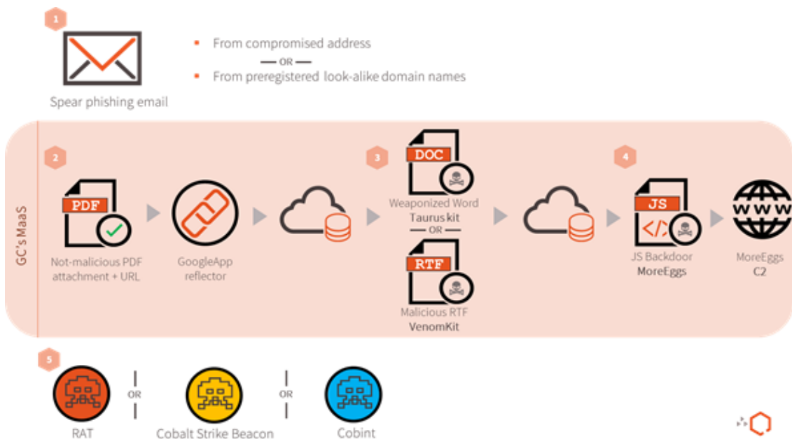
Figure 5 — Cobalt and GC campaigns using the Provider
