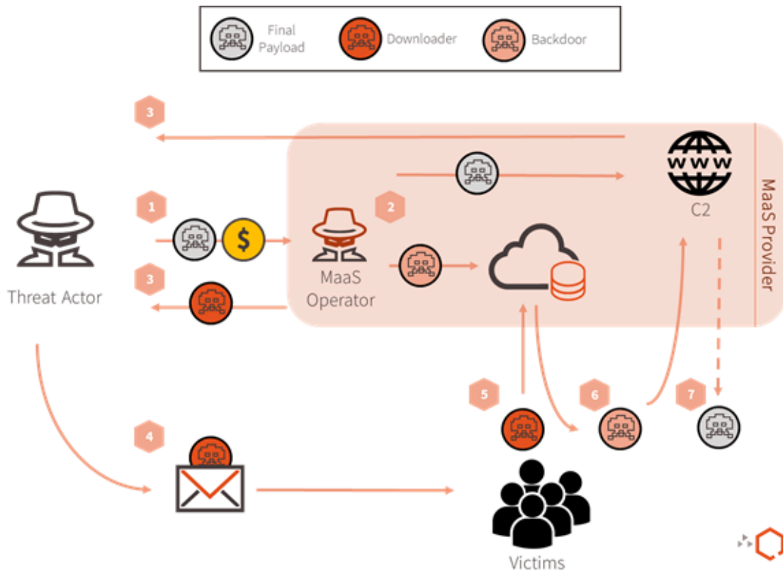
Figure 2 –The Provider operational workflow
