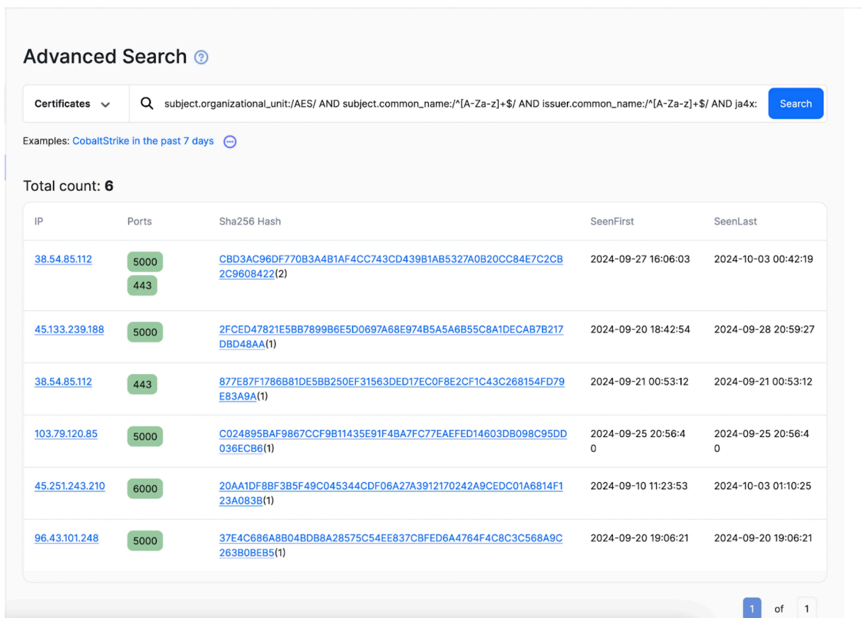
Figure 1: Query results for suspicious PlugX certificates. Search conducted on 03 October ( Hunt Link )
