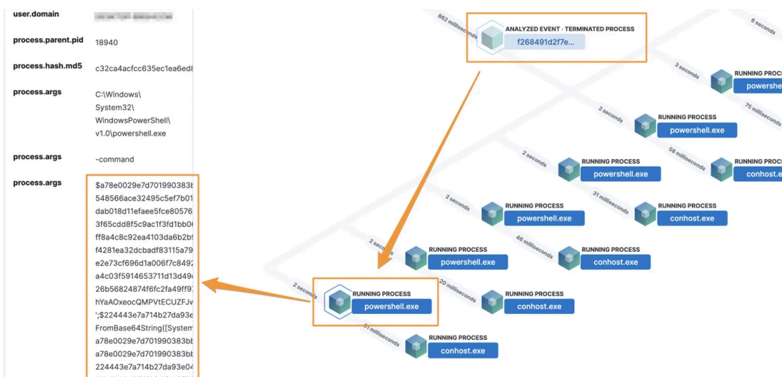
Figure 15: Malware executing obfuscated PowerShell processes
