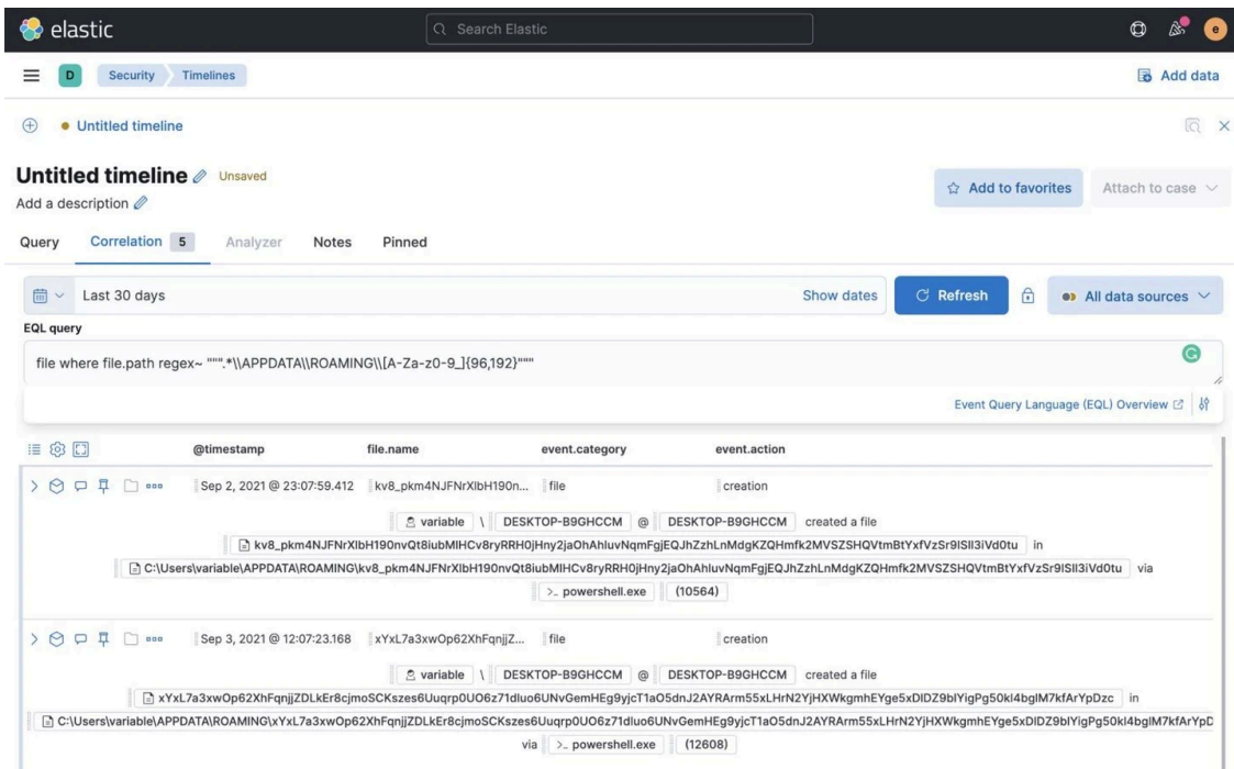
Figure 19: Hunt query identifying Hardware ID using Timelines
