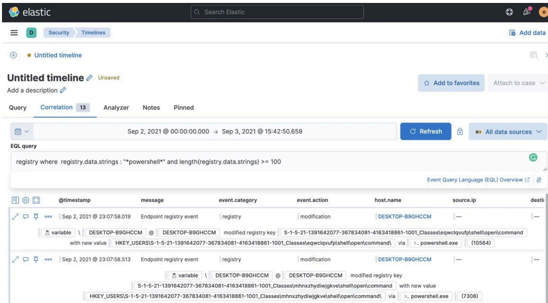
Figure 23: Hunt query identifying long Registry strings in Timelines
