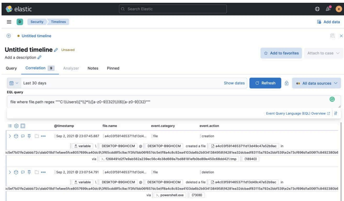
Figure 17: Hunt query identifying initial installer using Timelines
