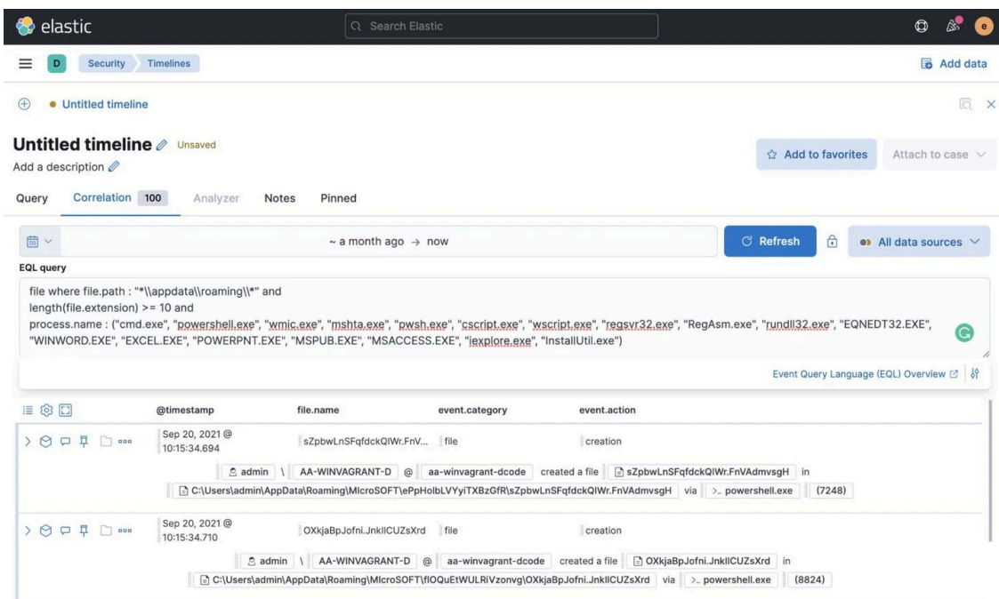
Figure 21: Hunt query identifying long file extensions in Timelines
