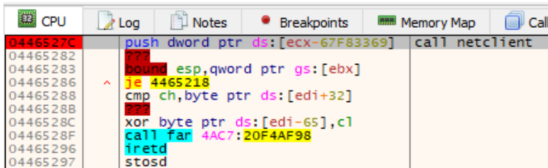
Figure 13 – If we try to view the code of the main module, i.e. go to the offset that called netclient , we can see that it no longer makes sense – as it was encrypted.
