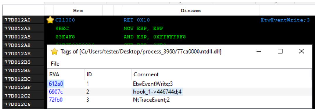
Figure 25 – Multiple patches in the NTDLL (32-bit), including the ones disabling ETW.
