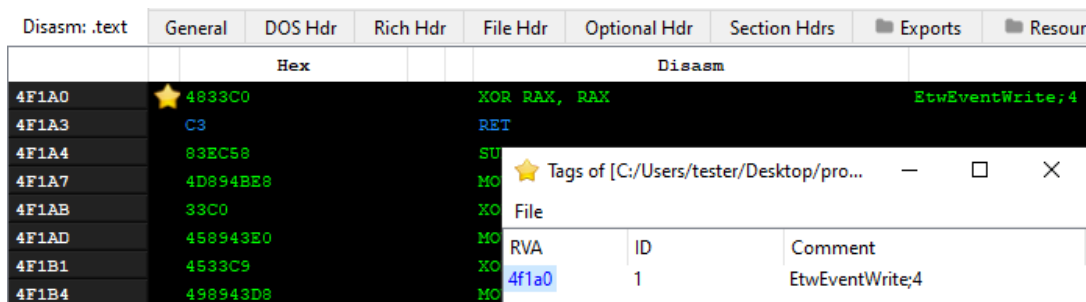
Figure 24 – The patch in the NTDLL (64-bit), disabling function EtwEventWrite.
