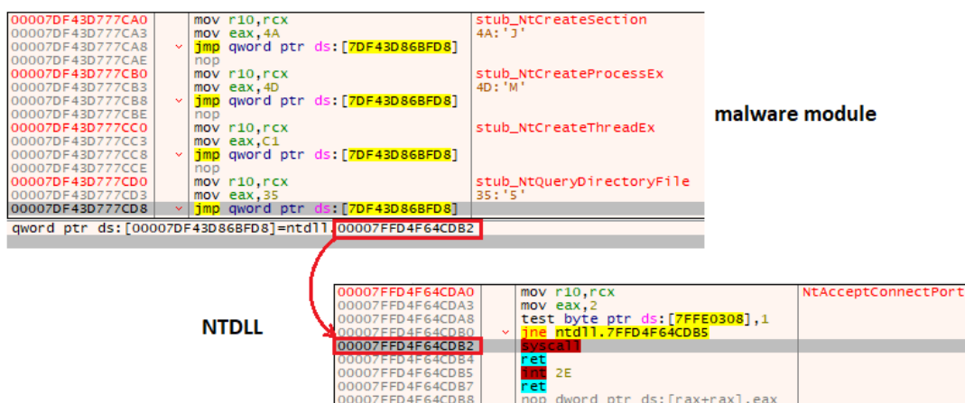
Figure 8 – Implementation of indirect syscalls used by Rhadamanthys.
