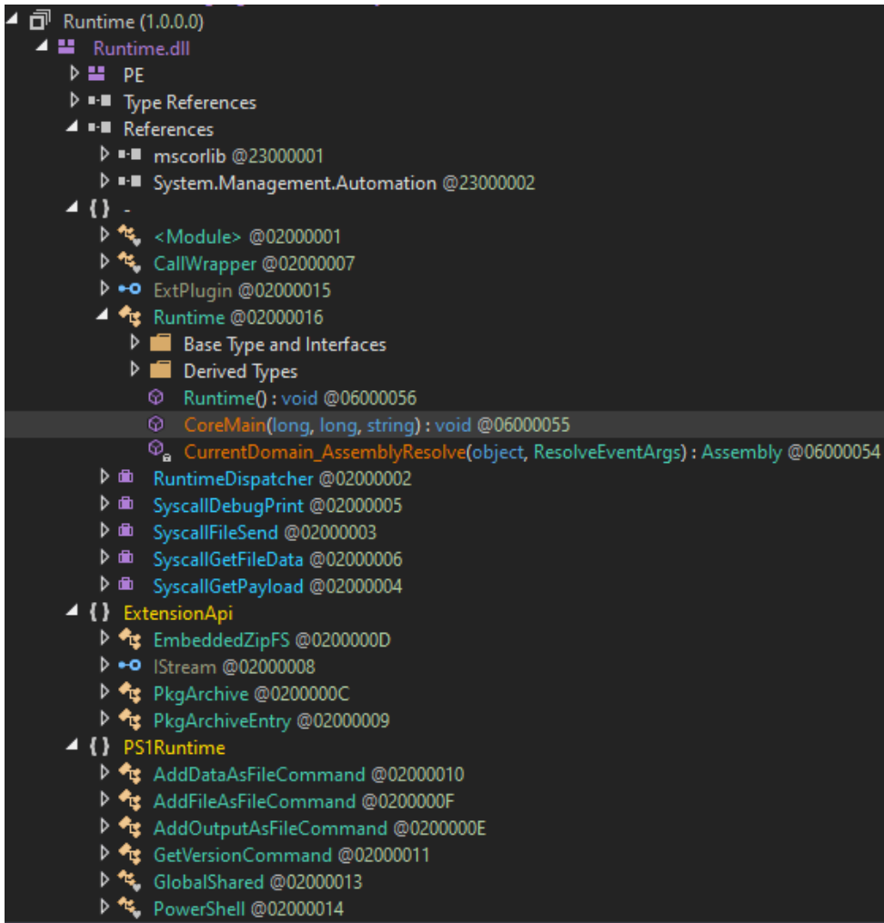
Figure 44 – List of classes on the runtime.dll (decompiled using dnSpy).
