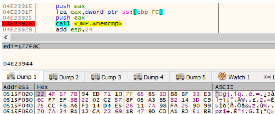
Figure 14 – The downloaded package after decryption
