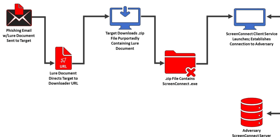
Figure 1 - Static Kitten Campaign Infection Chain
