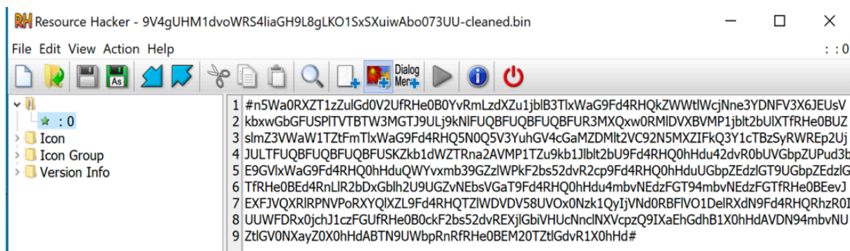
Figure 9: Encrypted configuration
