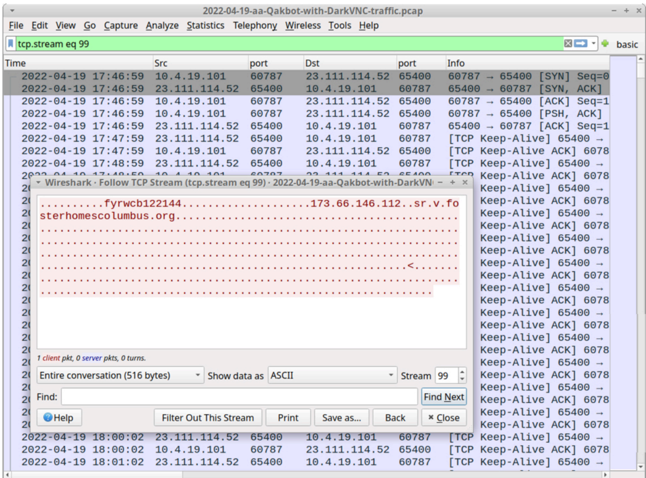
Shown above: Qakbot traffic on 23.111.114[.]52 over TCP port 65400.
