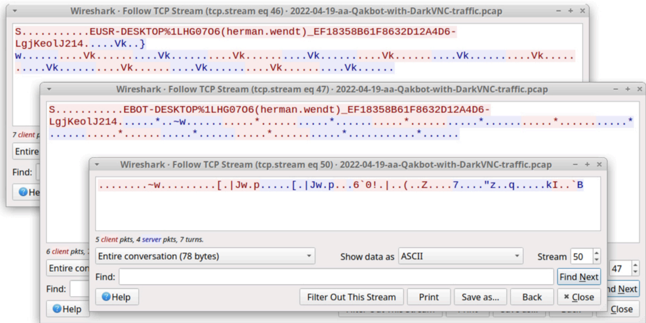
Shown above: TCP streams for DarkVNC traffic on 45.153.241[.]142 over TCP port 443.
