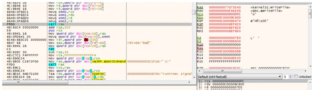
Figure 15 – WriteFile All these functions are called one after another, till all the files are encrypted. After encrypting the file, the key is stored at the end of the file.
