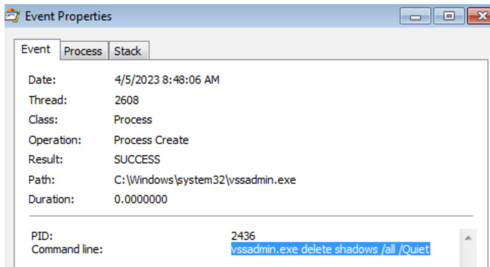
Figure 9 – Delete
