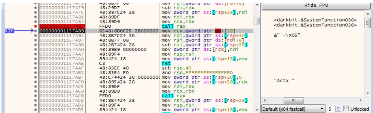
Figure 10 – SystemFunction036
