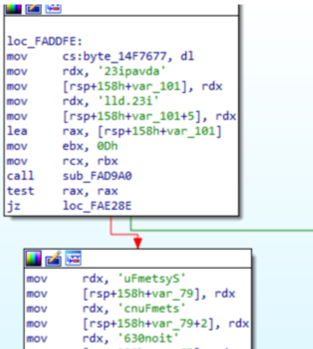
Figure 7- Obfuscation
