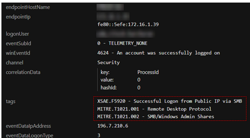
Figure 4. Successful initial entry for Prometei
