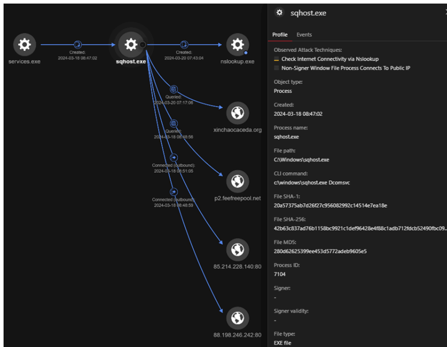
Figure 14. Sqhst.exe activity detected by Vision 1 Execution Profile
