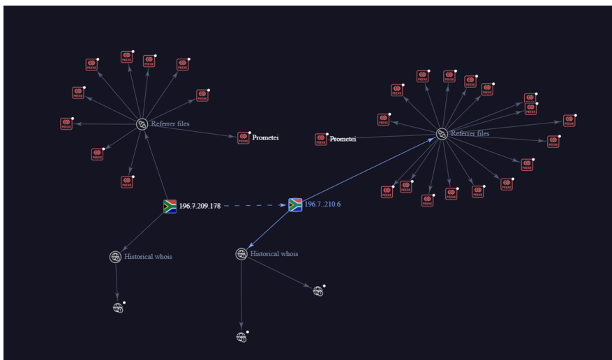
Figure 2: Relationship between IPs observed and Prometei Malware
