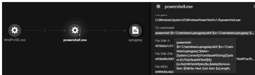
Figure 8. PowerShell decoded the Base64-encoded files (*.b64 file extension) to a new file.
