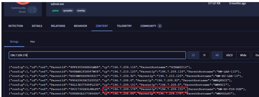
Figure 3: Hardcoded IP inside Prometei variant
