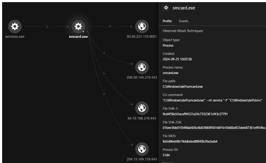
Figure 18. Smcard.exe acts as a TOR relay
