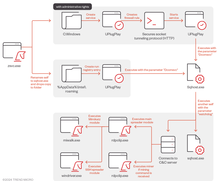
Figure 19. Prometei installation routine
