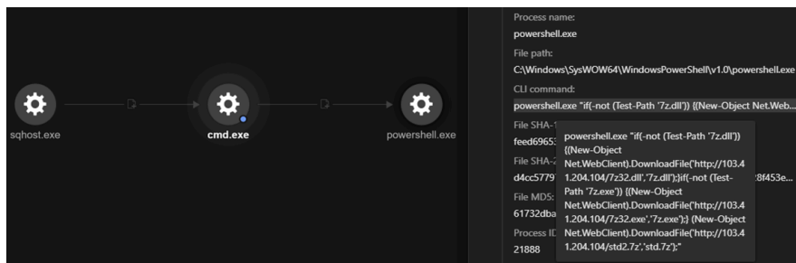
Figure 10. PowerShell downloads additional files from 103[.]41[.]204[.]104
