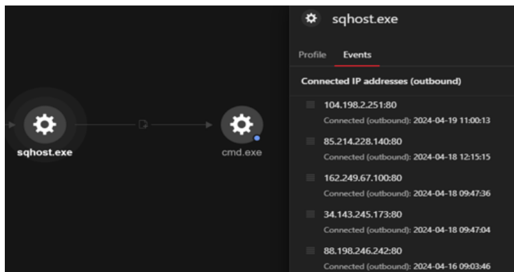
Figure 9. Sqhost.exe connection to 88.198.246[.]242
