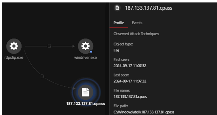
Figure 11. rdclip.exe reads the contents of .cpass
