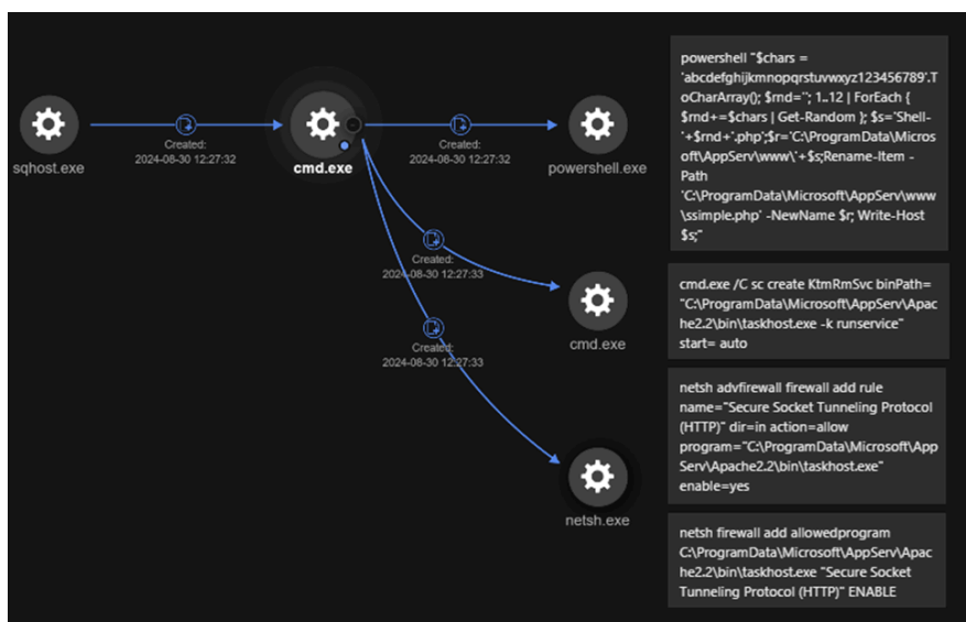
Figure 15. Sqhst.exe activity detected by Vision One execution profile
