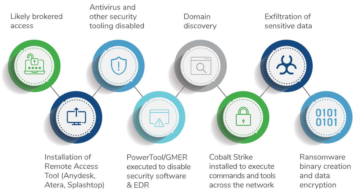
Figure 1 - Tactics, Techniques and Procedures (TTPs) of Recent Royal Ransomware Investigation
