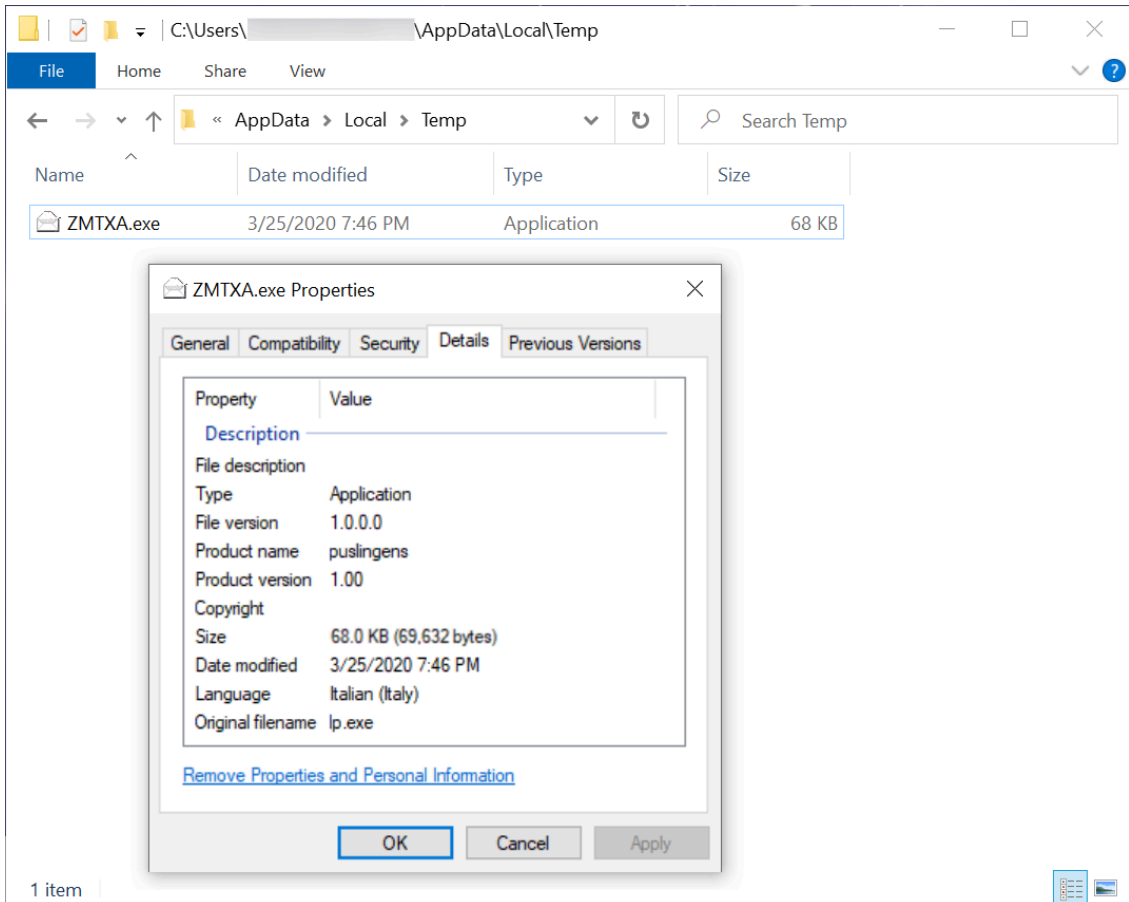
Figure 7. Binary for GuLoader after enabling macros on Andys_18US_Tax.doc
