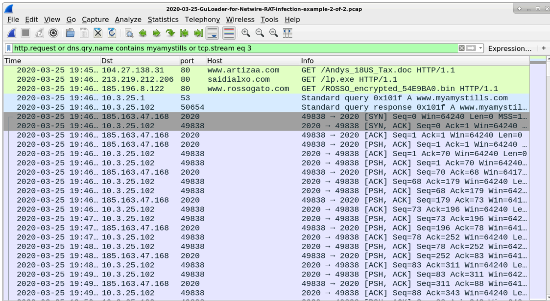
Figure 9. NetWire RAT infection traffic associated with PM_2019_Screen_18_Tax_File.doc and GuLoader filtered in Wireshark
