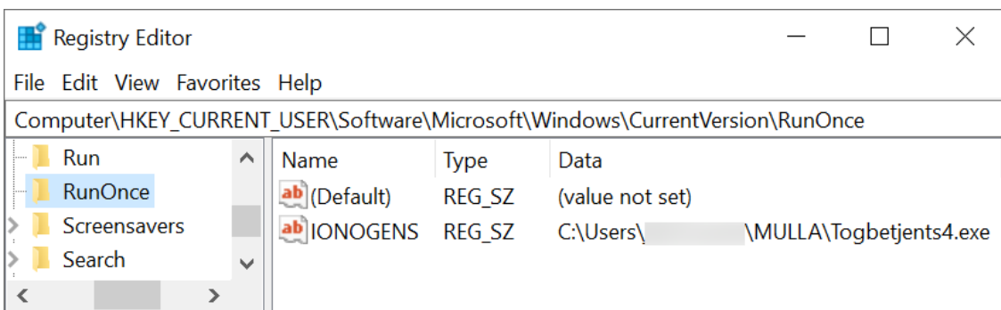
Figure 11. First example of GuLoader persistent through the Windows Registry.
