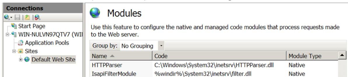
Figure 2 Installed RGDoor module displayed in the HTTP Modules list in IIS Manager
