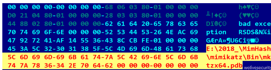
Figure 5. A PDB string in the Mimikatz payload
